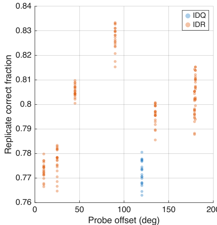
Upstream-noise hard-max choices (20 replicates)
